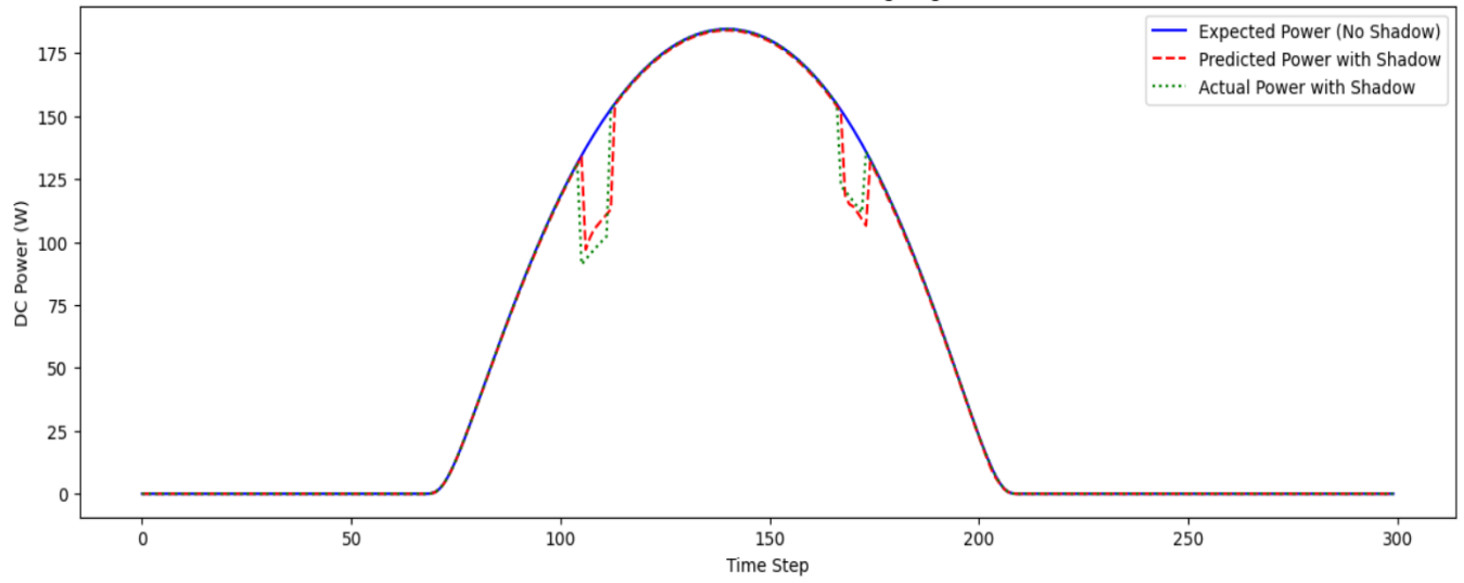
Predicted vs Actual Power Loss Due to Shading (Nighttime Handled)
